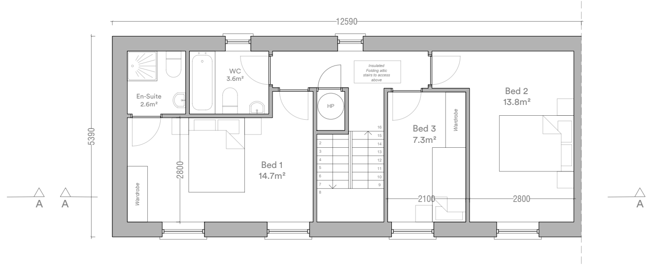
House Type O1/O2 First Floor Plan 55m 2
