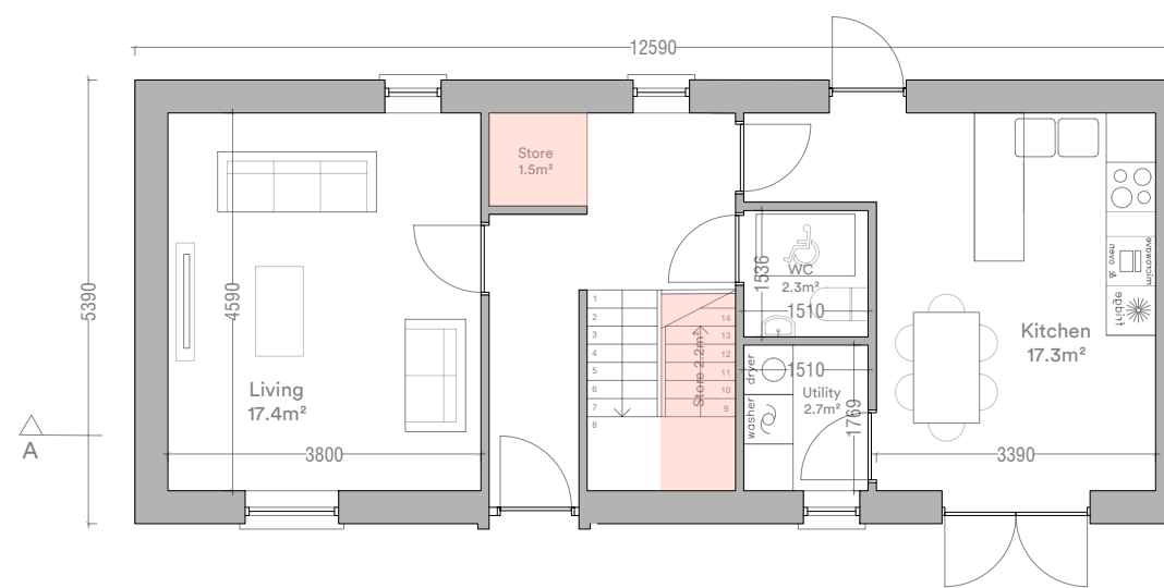
House Type O1/O2 Ground Floor Plan 55m 2
